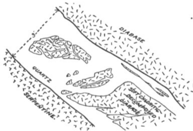
Figure 7: #1 Vein Cross Section, Section looking East (Lindgren, 1896)
