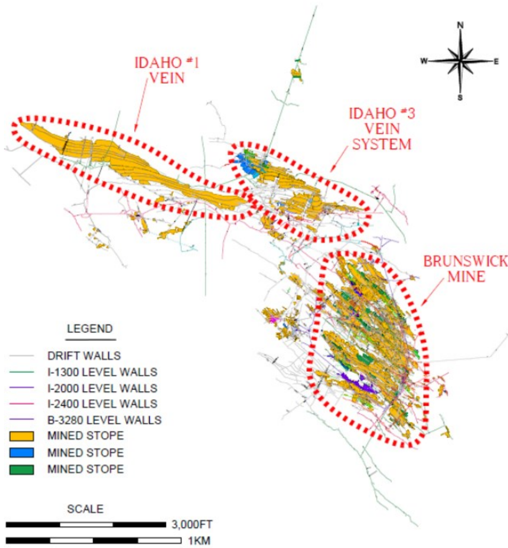
Figure 6: Idaho-Maryland Mine Workings, Plan View
